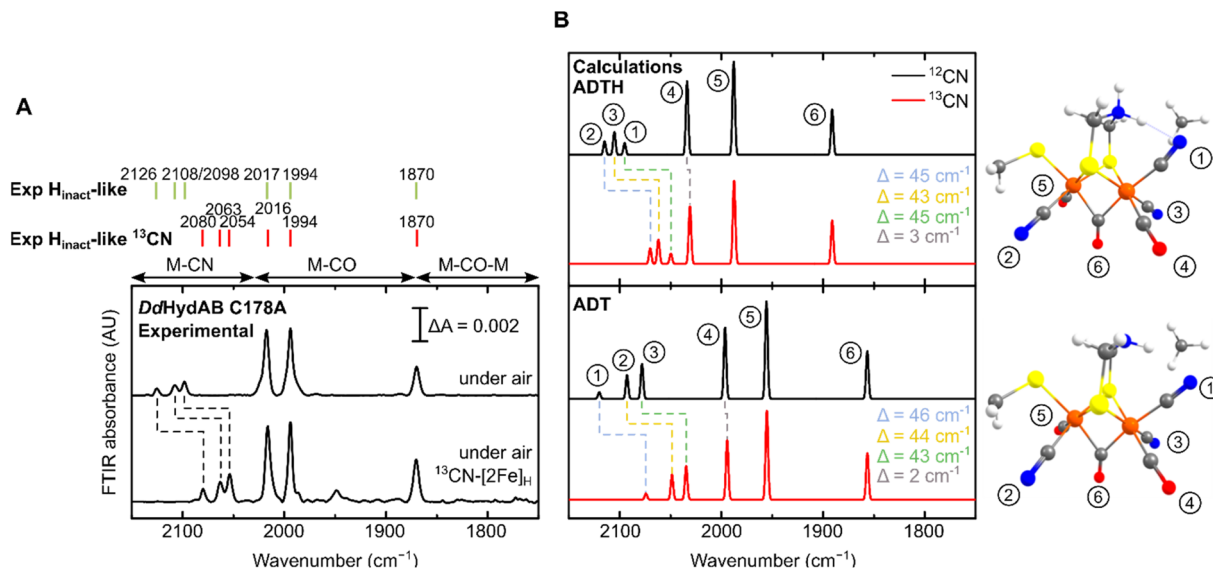
Fig. 3 (A) Experimental IR spectra of DdHsdAB C178A matured with natural abundance (top) and ^{13}\text{CN}^- -labeled [2\text{Fe}]_{\text{H}} precursor (bottom), both exposed to air to form the \text{H}_{\text{inact}} -like state. The small additional feature in the ^{13}\text{CN} spectrum may represent a small amount of an unknown degradation product. (B) Calculated IR spectra of the H-cluster model with either a singly protonated (ADT) or doubly protonated (ADTH) ADT ligand. Insets are [2\text{Fe}]_{\text{H}} structures with chemical groups associated with modes labelled. A scaling factor of 0.964 was used.
