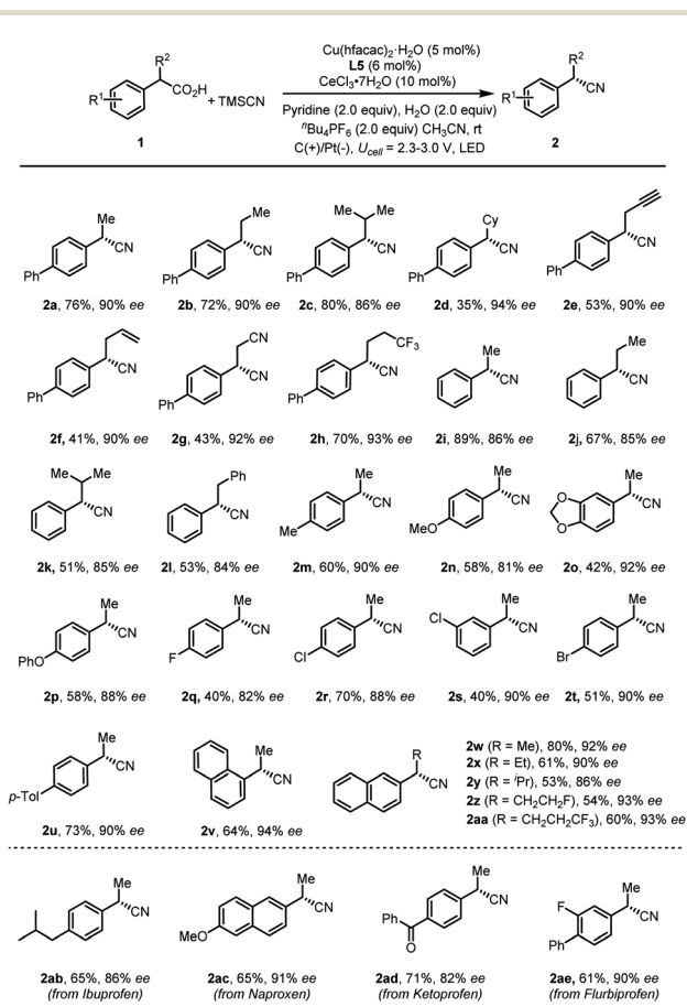
Scheme 2 Scope of carboxylic acids. The reaction was performed on a 0.2 mmol scale under the conditions in Table 1, entry 1.
