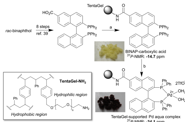
Scheme 1 Reagents and conditions: (a) TentaGel-NH 2 , EDCI, HOBT, DMF, retention time of 13 h. (b) [Pd(CH 3 CN) 4 ] 2+ (TfO − ) 2 , wet acetone, retention time of 7 h, 96% in 2 steps.
