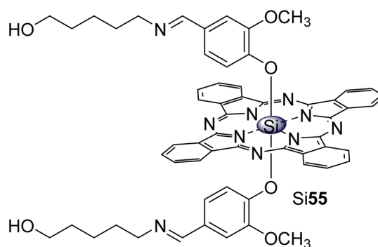
Fig. 28 Silicon phthalocyanine Si55 used by Anucha, Altin and co-workers 193 for the degradation of carbamazepine.
