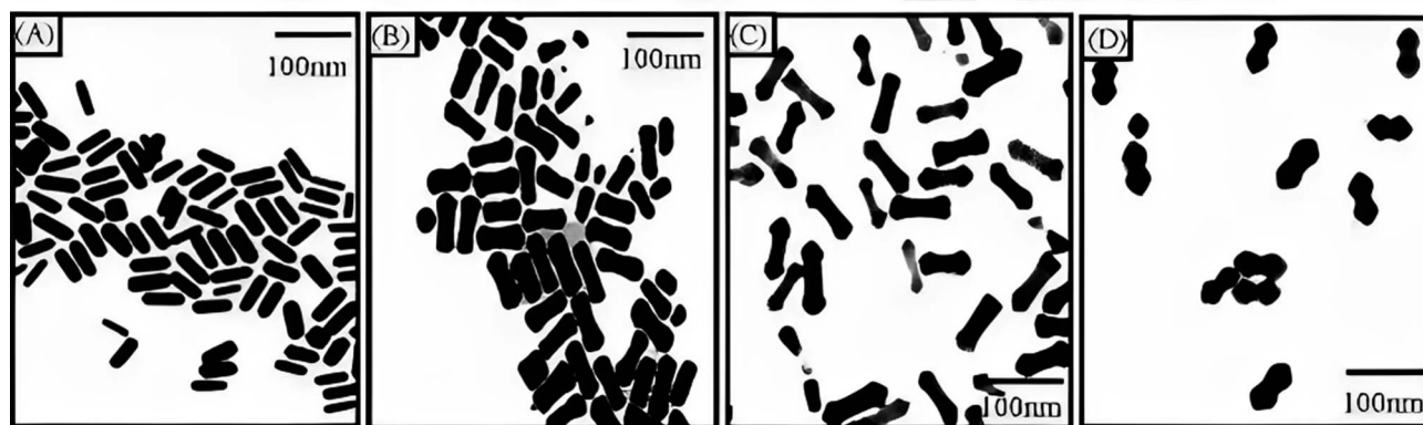
Fig. 8 (a) TEM of (GNR), (b) Au@Ag with thin composite NRs, and (c) thick thin composite NRs with Ag layers. Permission from ref. 127 © 2001 American Chemical Society. Image bottom: (A) TEM of (GNR) as prepared, and (B) Au@Ag composite NRs prepared at the alkaline solution of surfactant at pH 8.0, (C) pH 9, and (D) pH 10 permission from ref. 125 © 2004 American Chemical Society.
