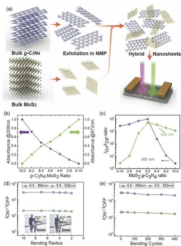
Fig. 5 (a) Schematic illustration of the process for preparation of g - C_3N_4 and MoS_2 hybrid dispersions used for photodetector; (b) absorbance at wavelengths of 672 nm and 308 nm and (c) on-off ratio as a function of the g - C_3N_4 and MoS_2 ratio. (d) On-off ratio of the photodetectors containing g - C_3N_4 and MoS_2 hybrid with different bending radius. (e) On-off ratio of the photodetectors containing g - C_3N_4 and MoS_2 hybrid with different bending cycles at a banding radius of \approx 4 mm. Reproduced from ref. 77 with permission. Copyright 2017, John Wiley and Sons Ltd.
