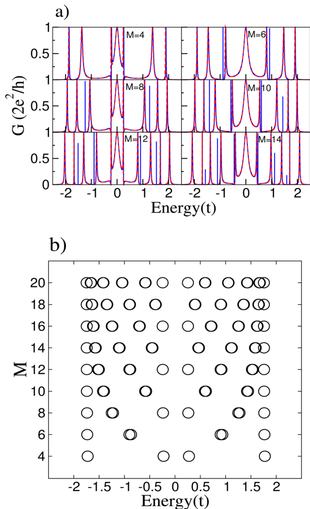
Fig. 4 (a) Conductance vs. energy for several rings in the polyynic configuration with an impurity of energy s = 0.1t (blue) and no impurity (red). (b) Energy spectra of the isolated rings from M = 4 to M = 20 with an impurity of energy s = 0.1t for the polyynic configuration in the tight-binding model.
