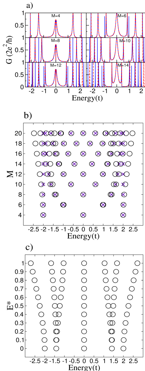
Fig. 5 (a) Conductance vs. energy for several rings in the cumulenic configuration with E^* = 0.2 (blue) and no electric field (red). (b) Energy spectra of the isolated rings from M = 4 to M = 20 for the cumulenic configuration in the tight-binding model with E^* = 0.2 (circle) and no electric field (X). (c) Variation in the energy spectra of the ring with M = 8 sites in the cumulenic configuration for several values of E^* .
