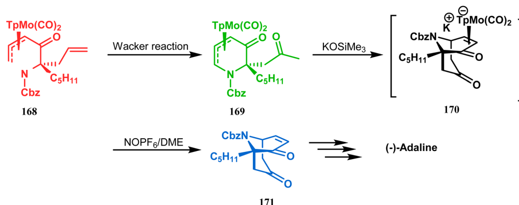
Scheme 33 Synthetic route for the formation of enantiomerically pure (–)-adoline.
