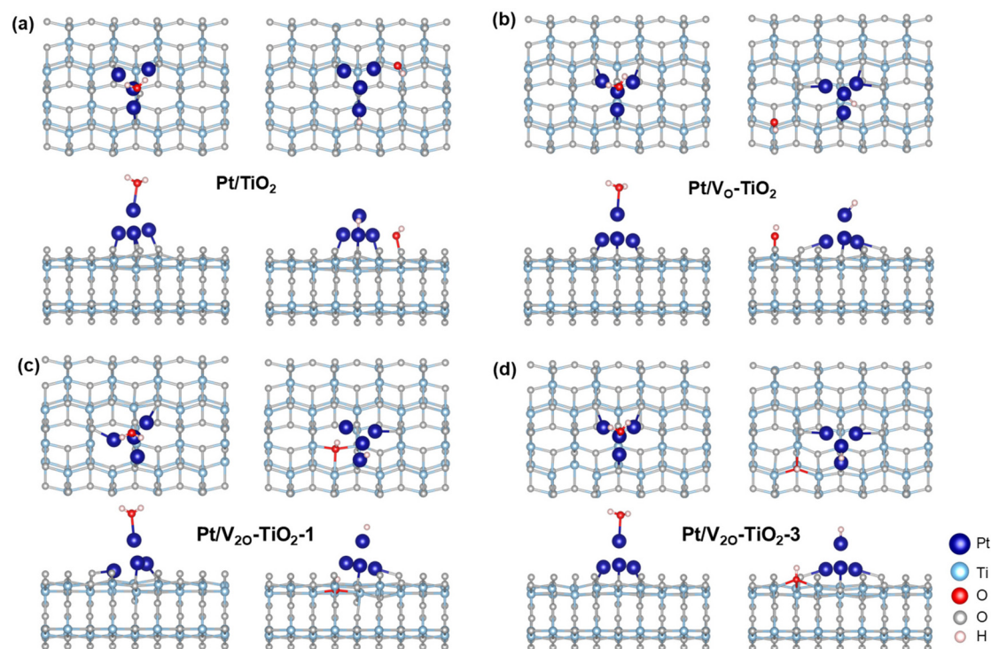
Fig. 6 Structures for \text{H}_2\text{O} and \text{OH}^*/\text{H}^* adsorbed on the (a) \text{Pt}/\text{TiO}_2 , (b) \text{Pt}/\text{V}_\text{O}-\text{TiO}_2 , (c) \text{Pt}/\text{V}_{2\text{O}}-\text{TiO}_2-1 , (d) \text{Pt}/\text{V}_{2\text{O}}-\text{TiO}_2-3 surfaces.
