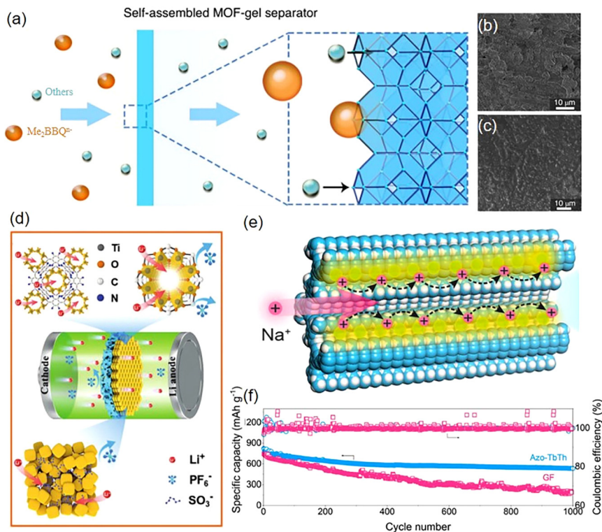
Fig. 24 (a) Schematic illustration of MOF-gel separator for limiting Me 2 BBQ - . Comparison of SEM images of the deposition morphology of lithium metal electrodes using a common separator (b) and MOF-gel separator (c). Reproduced with permission. 216 Copyright 2020, Springer Nature. (d) Schematic diagram of MOFs@PP separator regulating Li + and anion migration in LMBs. Reproduced with permission. 217 Copyright 2021, Wiley-VCH GmbH. (e) Schematic profile of Na + rapid migration mechanism in Azo-TbTh separator. (f) Cyclic stability of Na-S batteries assembled with Azo-TbTh and GF as separators at 1 C. Reproduced with permission. 220 Copyright 2022, the American Chemical Society.
