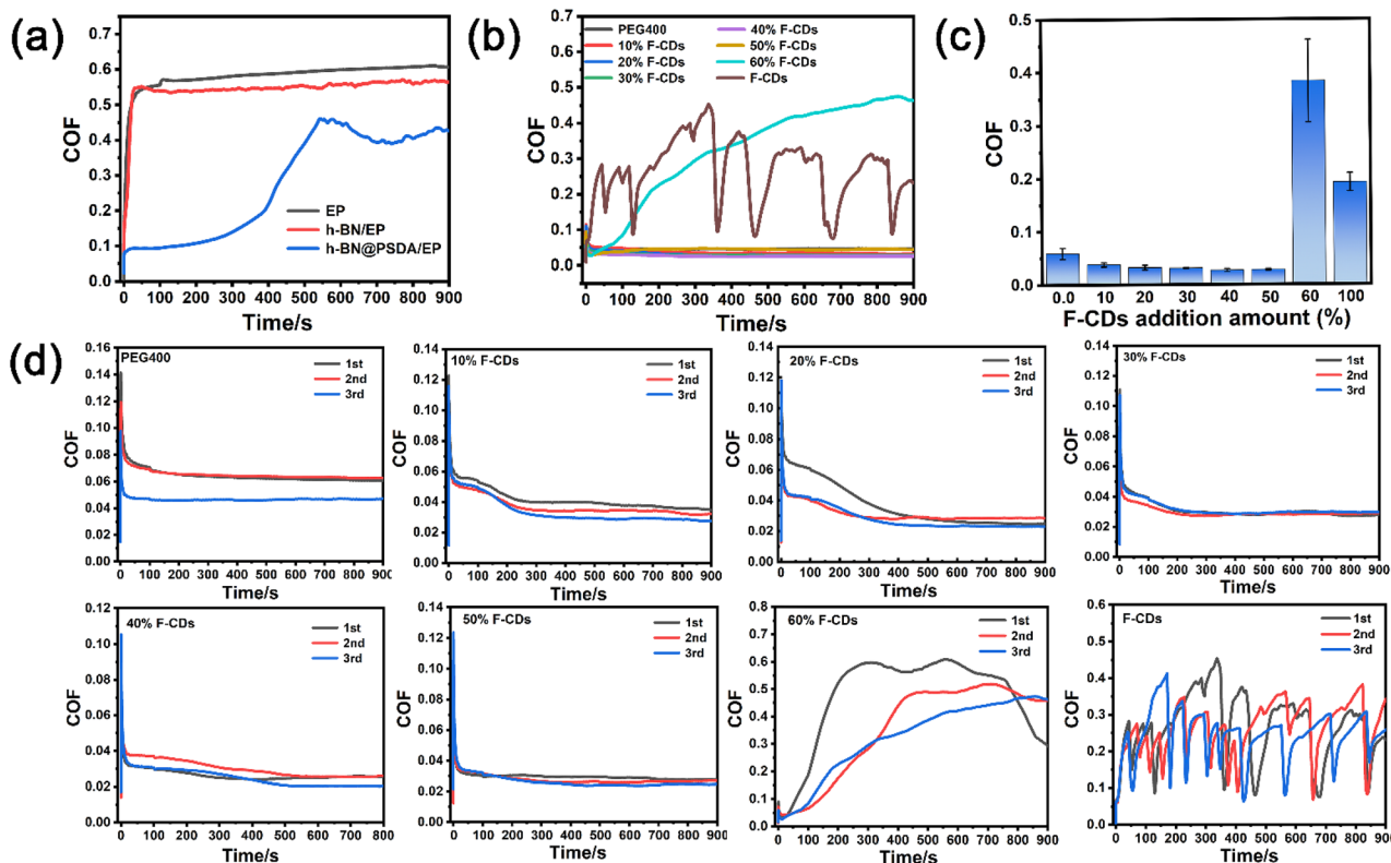
Fig. 6 (a) The coefficient of friction curves of EPs, h-BN/EPs and h-BN@PSDA/EPs, respectively, under dry conditions. (b) The coefficient of friction curves of F-CDs dissolved in PEG 400 at concentrations of 10 wt%, 20 wt%, 30 wt%, 40 wt%, 50 wt%, and 60 wt%, respectively, and (c) the corresponding histograms. (d) The coefficient of friction curves for repeated tests of F-CDs in PEG400 at concentrations of 10 wt%, 20 wt%, 30 wt%, 40 wt%, 50 wt%, and 60 wt%, respectively.
