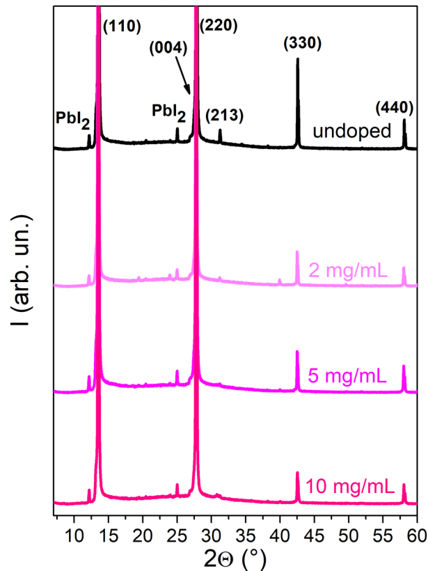
Fig. 4 XRD spectra of the undoped MAPI film and MAPI doped with concentrations of 2–10 \text{mg mL}^{-1} . For higher doping concentrations, see Fig. S9 (ESI \dagger ).
