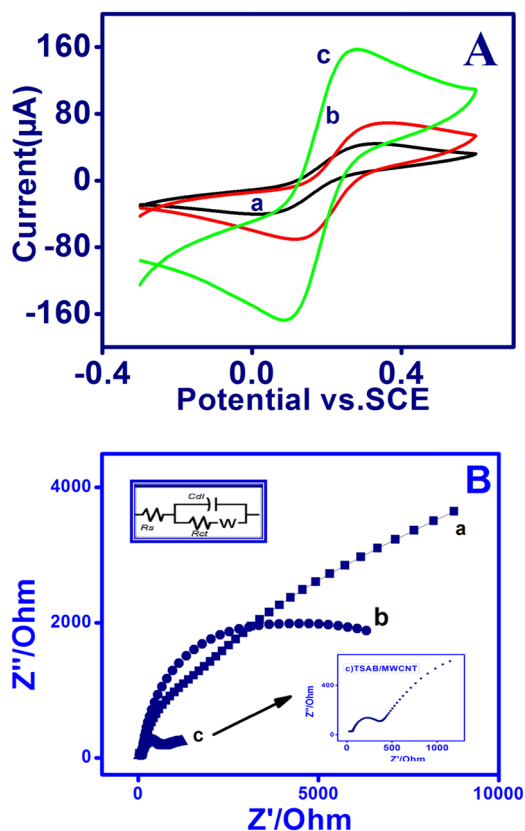
Fig. 2 (A) Cyclic voltammograms and (B) electrochemical impedance spectra on PIGE (curve a ), MWCNT (curve b ) and TSAB/MWCNT (curve c ) in 1 mM [Fe(CN) 6 ] -3/4- containing 0.1 mol L -1 ABS (pH-5.0) at 50 mV s -1 . Inset: Enlarged image of (B) depicting the EIS of TSAB/MWCNT-modified electrode.
