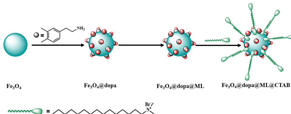
Scheme 6 Schematic representation of the synthesis of bilayer \text{CTAB}/\text{Fe}_3\text{O}_4@\text{dopa}@FeL (CHCAT-1) and \text{CTAB}/\text{Fe}_3\text{O}_4@\text{dopa}@MnL (CHCAT-2).
