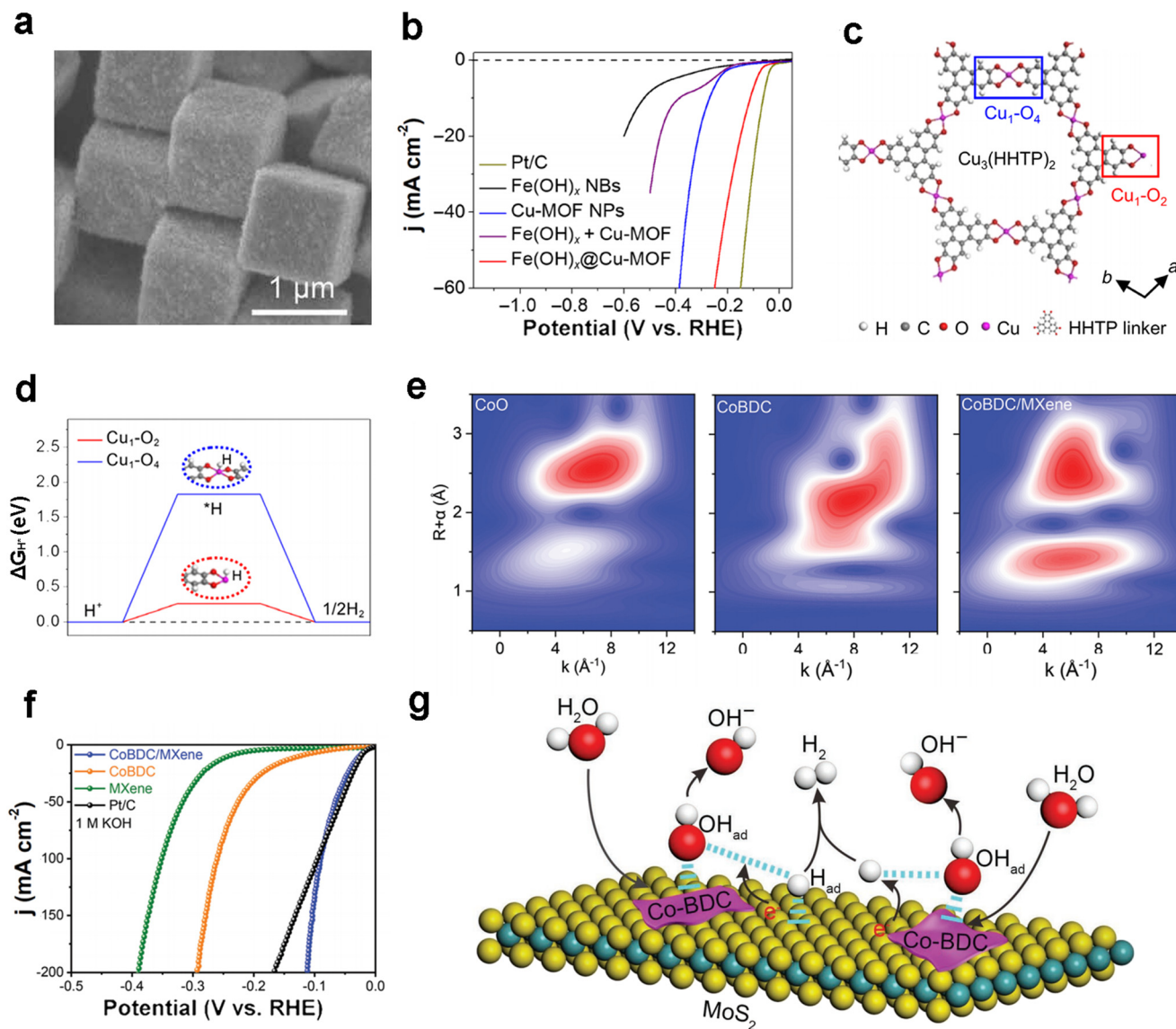
Fig. 2 MOF-based HER electrocatalysts. (a) FESEM images of sample \text{Fe(OH)}_x\text{@Cu-MOF NBs} ; (b) LSV curves of Pt/C, \text{Fe(OH)}_x NBs, Cu-MOF NPs, \text{Fe(OH)}_x + \text{Cu-MOF} , and \text{Fe(OH)}_x\text{@Cu-MOF NBs} in 1.0 M KOH; (c) crystal structure of unsaturated Cu-MOF[ \text{Cu}_3(\text{HHTP})_2 ] observed along the c -axis; (d) \Delta G of adsorbed ^*\text{H} calculated at the Cu sites of \text{Cu}_1\text{-O}_4 and \text{Cu}_1\text{-O}_2 centers. Reproduced with permission. 44 Copyright 2021, American Association for the Advancement of Science; (e) wavelet transform plots of k^3 -weighted EXAFS signals for CoO, CoBDC and CoBDC/MXene; (f) LSV curves of Pt/C, MXene, CoBDC and CoBDC/MXene for HER tests in 1.0 M KOH. Reproduced with permission. 45 Copyright 2022, Wiley-VCH; (g) schematic diagram of the basic HER catalytic mechanism of the Co-BDC/ \text{MoS}_2 composite. Reproduced with permission. 46 Copyright 2019, Wiley-VCH.
