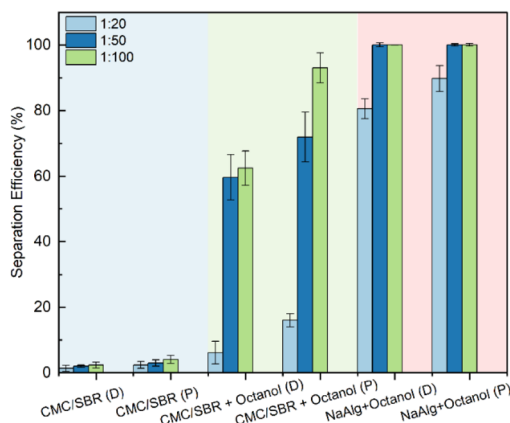
Fig. 6 Separation efficiencies of the samples involved in this project in an ultrasonic time of 10 minutes, with an active material to solvent ( i.e. distilled water in this case) ratio of 1:20, 1:50 and 1:100 respectively. Here D is short for draw-down electrodes, P is short for printed electrodes.
