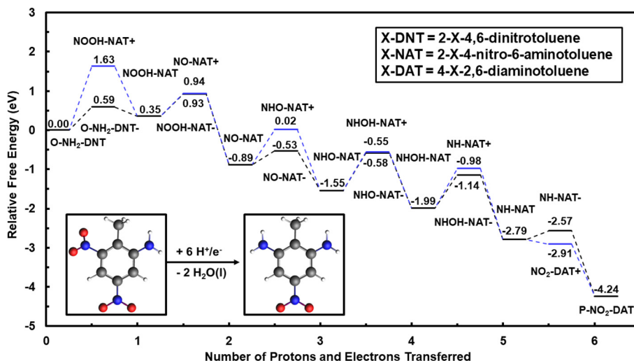
Fig. 2 Reaction energy diagram for outer-sphere electrochemical reduction of \text{O-NH}_2\text{-DNT} to \text{P-NO}_2\text{-DAT} in the solution phase, calculated using the G16 code and IEFFPCM solvation model. Reduction proceeds by reducing the second ortho \text{NO}_2 group to the methyl group of TNT. Energies are relative to \text{O-NH}_2\text{-DNT} in the solution phase at 0 V-NHE and \text{pH} = 0 . Water molecules formed during the TNT reduction are not shown for clarity purposes. Black lines represent reduction steps initiated by uncoupled electron transfer followed by proton transfer. Blue lines represent reduction steps initiated by uncoupled proton transfer followed by electron transfer. Atom colors are presented as grey: C, white: H, blue: N, and red: O.
