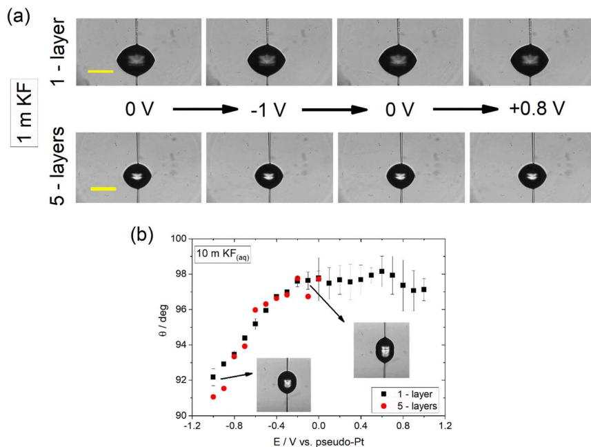
Fig. 2 (a) Images of 1 m \text{KF}_{(\text{aq})} droplets on CVD graphene of 1- (top row) and 5- (bottom row) layers at varied applied potentials. The scale bars correspond to 200 \mu\text{m} . (b) Change in apparent equilibrium electrowetting contact angle, \theta , with the applied bias (values are reported vs. Pt wire pseudo-reference electrode) at the CVD graphene|10 m \text{KF}_{(\text{aq})} interface for 1- and 5-layers thickness. Measurements were conducted under static conditions based on the protocol described in the Experimental section.
