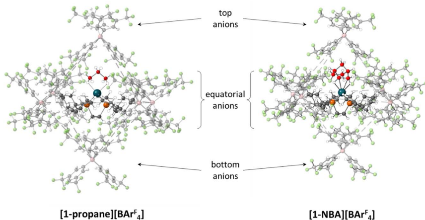
Fig. 1 Packing diagrams showing the pseudo-octahedral arrangement of [\text{BARF}_4]^- anions around the Rh cations in [1\text{-NBA}][\text{BARF}_4] and [1\text{-propane}][\text{BARF}_4] . Carbon atoms of the \sigma -alkane ligands are highlighted in red.
