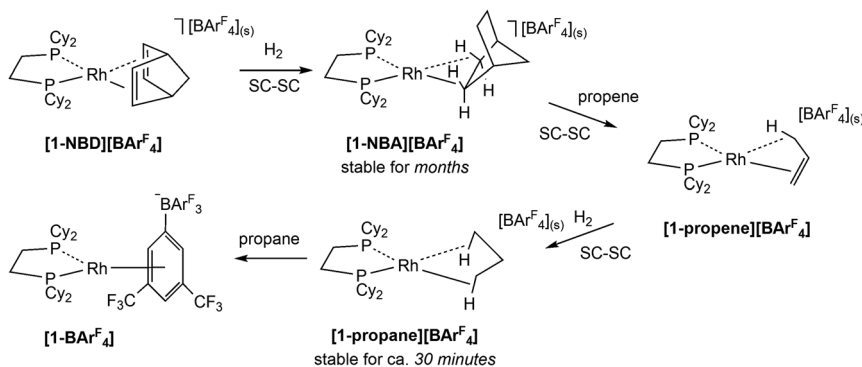
Scheme 1 Synthesis of \sigma -alkane complexes via single crystal-to-single crystal (SC–SC) transformations: (a) [1\text{-NBA}][\text{BAR}^F_4] by hydrogenation of [1\text{-NBD}][\text{BAR}^F_4] ; (b) [1\text{-propane}][\text{BAR}^F_4] from [1\text{-NBA}][\text{BAR}^F_4] via sequential NBA/propene substitution and hydrogenation.
