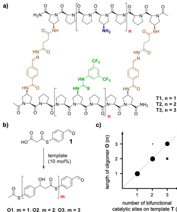
Fig. 1 (a) Catalytic macrocyclic templates T1–T3; (b) catalytic length-controlled oligomerization of malonic acid half thioester (MAHT)-aldehyde bifunctional substrate 1 ; and (c) correlation between the number of catalytic sites on the template with the length of the formed oligomer.
