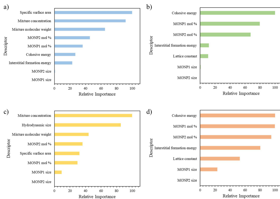
Fig. 8 Relative importance of descriptors in random forest (RF)-based models predicting \log EC_{50} (Fig. 8a and b) and \log EC_{10} (Fig. 8c and d). All descriptor-based models (Fig. 8a and c) and calculated descriptor-based models (Fig. 8b and d).
