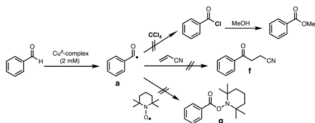
Scheme 5 Acyl radical trapping experiments.
