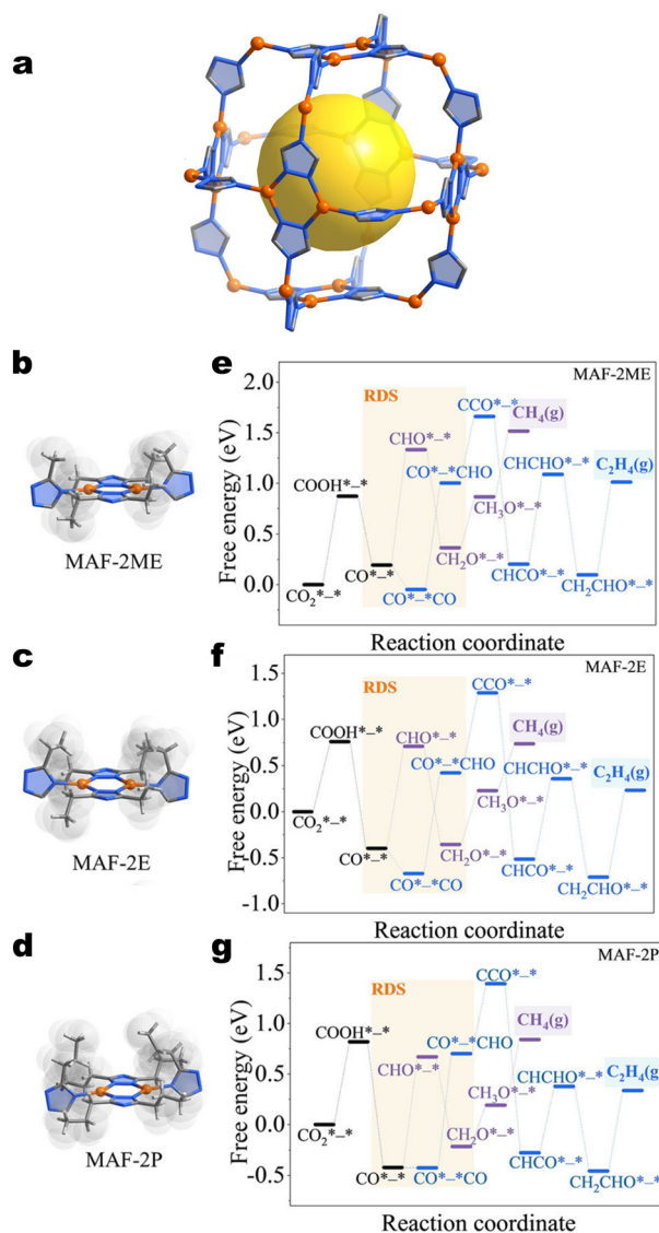
Fig. 20 Structures of MAF-2 analogues a) the Cu(I) triazolate backbone with ligand side groups omitted. Local coordination environments of b) MAF-2ME, c) MAF-2E, and d) MAF-2P. Orange spheres denote copper atoms. Blue, grey, and white edges denote nitrogen, carbon, and hydrogen atoms. Orange spheres denote copper atoms. Free energy diagrams for CH 4 and C 2 H 4 formation on e) MAF-2ME, f) MAF-2E, and g) MAF-2P. Reproduced with permission from Zhuo et al. 131 Copyright 2022 John Wiley & Sons, Inc.
