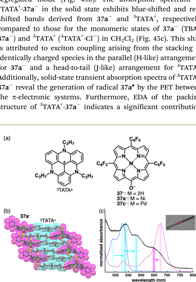
Fig. 45 (a) Ion pairs ^3TATA^+-37^- and ^3TATA^+-37a,c^- , (b) single-crystal X-ray structure of ^3TATA^+-37a^- (redrawn from a cif file: 1906678) and (c) UV/vis absorption spectrum of the single crystal of ^3TATA^+-37a^- (black) along with those of the solution states ( 1 \times 10^{-5} M in CH_2Cl_2 ) of TBA^+-37a^- (magenta) and ^3TATA^+-Cl^- (cyan) (inset: optical microscopy image of a single crystal of ^3TATA^+-37a^- ) (redrawn from ref. 9. Copyright 2021 RSC).
