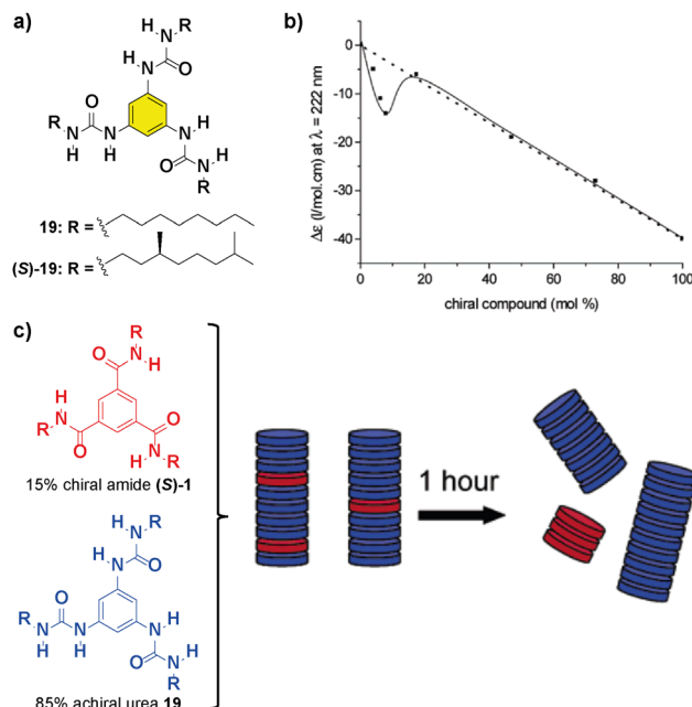
Fig. 12 (a) Chemical structure of benzene trisreas 19 . (b) SaS experiment between chiral (S)-1 and achiral 19 ( c_T = 50 \mu\text{M} in heptane). (c) Schematic representation of the aggregates formed during the mixing of 15% of (S)-1 and 85% of 19 (reproduced from ref. 82 with permission from the American Chemical Society, copyright 2022).
