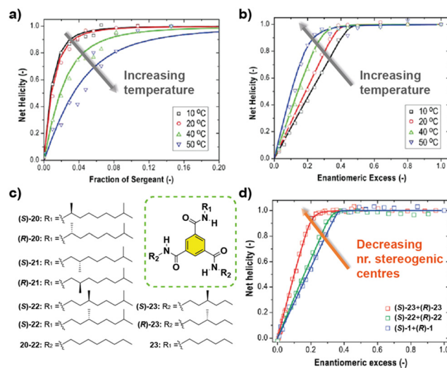
Fig. 13 SaS (a) and MR (b) experiments of (S)-1 and (R)-1 at different temperatures ( c_T = 20 \mu\text{M} in MCH). (c) Chemical structure of asymmetric BTAs. (d) MR experiments with BTAs containing a different number of stereogenic centres ( c_T = 30 \mu\text{M} in MCH) (reproduced from ref. 77 and 78 with permission from the American Chemical Society, copyright 2010).
