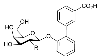
105 R = \text{OH} K_D = 2.1 \mu\text{M} 106 R = \text{NHAc} K_D = 89 \text{ nM} , \text{IC}_{50} = 0.64 \mu\text{M}
