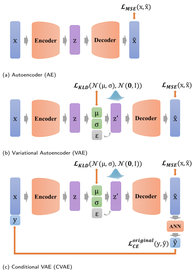
Fig. 4 Existing VAE structures.
