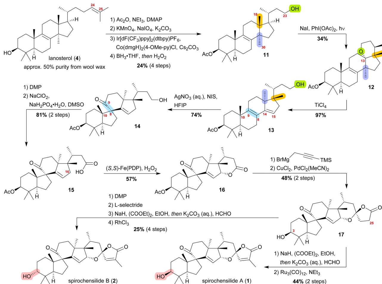
Scheme 2 Semisyntheses of spirochensilide A (1) and B (2) by Heretsch and co-workers. ppy = 2-phenylpyridine, dtbpy = 4,4'-di- t -butyl-2,2'-bipyridine, dmgh = dimethylglyoximate, (S,S)-PDP = (–)-2-(2-((S)-2-((S)-1-(pyridin-2-ylmethyl)pyrrolidin-2-yl)pyrrolidin-1-yl)methyl)pyridine.
