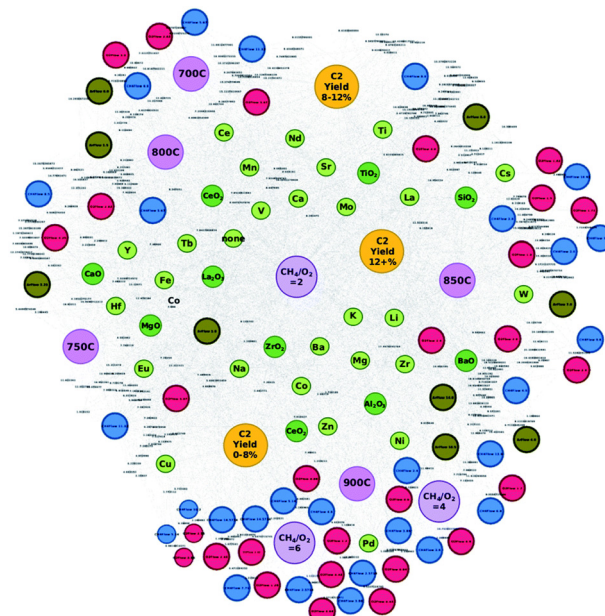
Fig. 13 Catalyst network using oxidative coupling of methane catalysts big data. The relationships between \text{C}_2 yield and composition and experimental conditions are unveiled. Reproduced from ref. 32 with permission from the Royal Society of Chemistry.
