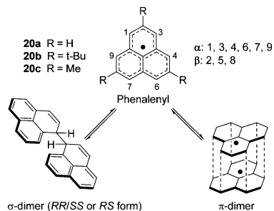
Fig. 16 Dimerization modes of 20 . Copyright 2016, American Chemical Society.
