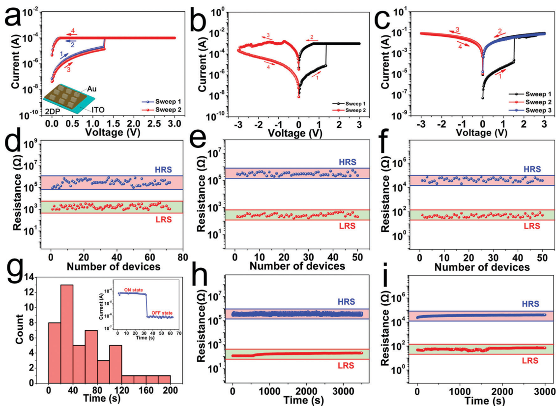
Fig. 3 (a, b and c) I - V characteristics of the Au/ 2\text{DP}_{\text{TPAK}+\text{TAPB}} /ITO device when the I_{\text{CC}} is 10^{-4}\text{ A} , 10^{-3}\text{ A} and 10^{-1}\text{ A} , respectively (inset: a schematic illustration of the Au/ 2\text{DP} /ITO device). (d, e and f) The device-to-device distributions of HRS resistance and LRS resistance (read at 0.1\text{ V} ) when the I_{\text{CC}} is 10^{-4}\text{ A} , 10^{-3}\text{ A} and 10^{-1}\text{ A} , respectively. (g) Retention time of the Au/ 2\text{DP}_{\text{TPAK}+\text{TAPB}} /ITO device when the I_{\text{CC}} is 10^{-4}\text{ A} (inset: I - t curve of the Au/ 2\text{DP}_{\text{TPAK}+\text{TAPB}} /ITO device). (h and i) Retention time of the Au/ 2\text{DP}_{\text{TPAK}+\text{TAPB}} /ITO device (read at 0.1\text{ V} ) when the I_{\text{CC}} is 10^{-3}\text{ A} and 10^{-1}\text{ A} , respectively. The thickness of the active layer ( 2\text{DP}_{\text{TPAK}+\text{TAPB}} ) of the above devices is about 20\text{--}30\text{ nm} .
