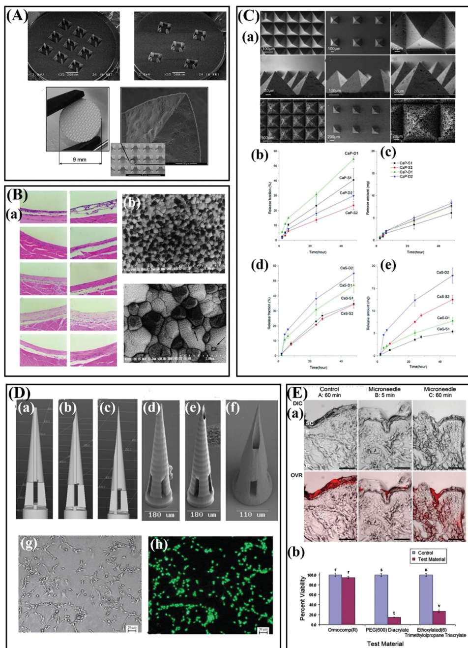
Fig. 5 (A) Overview images and detailed scanning electron micrographs of alumina-based nanoporous ceramic MNs. Adapted with permission from ref. 57. Copyright 2015 Elsevier. (B) (a) Tissue response around tested materials. (b) Scanning electron micrographs of Ce-TZP/Al 2 O 3 nanocomposite after thermal etching. Adapted with permission from ref. 59. Copyright 2002 John Wiley and Sons. (C) (a) SEM images: top view of intact calcium sulfate (CaS) MNs. (b) Fraction of drug released versus time and (c) amount of drug released versus time from CaP SCMN with zolpidem tartrate integrated into the matrix. (d) Fraction of drug released versus time and (e) amount of drug released versus time for CaS SCMN with zolpidem tartrate integrated into the matrix. Adapted with permission from ref. 63. Copyright 2012 Royal Society of Chemistry. (D) Computer-aided design diagrams of MNs with (a) 0 μm, (b) 1.4 μm, and (c) 20.4 μm pore–needle center displacement values. Scanning electron micrographs of Ormocer ® MNs with (d) 0 μm, (e) 1.4 μm, and (f) 20.4 μm pore–needle center displacement values. Adapted with permission from ref. 66. Copyright 2007 John Wiley and Sons. (g) Optical micrograph and (h) fluorescence micrograph of live/dead assay-stained B35 neuroblast-like cells on an Ormocer ® surface 48 h after inoculation. Adapted with permission from ref. 65. Copyright 2006 Elsevier. (E) MTT viability of human epidermal keratinocytes on Ormocomp ® , PEG (600) diacrylate, and ethoxylated (6) trimethylolpropane triacrylate surfaces relative to paired controls. Adapted with permission from ref. 68. Copyright 2010 American Scientific Publishers.
