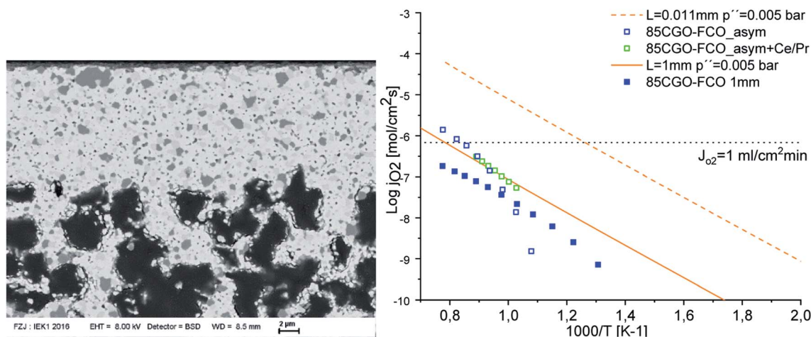
Fig. 27 Left: 11 \mu\text{m} thin asymmetric membrane made of \text{Ce}_{0.8}\text{Gd}_{0.2}\text{O}_{2-\delta} - \text{FeCo}_2\text{O}_4 composite (CGO-FCO) right: performance of asymmetric CGO-FCO with porous LSCF top-coating as well as advanced surface activation using (\text{Ce,Tb})\text{O}_2 - \text{NiFe}_2\text{O}_4 composite porous top coating and a Ce/Pr-based catalyst infiltrated into both top coating and porous CGO-FCO support.
