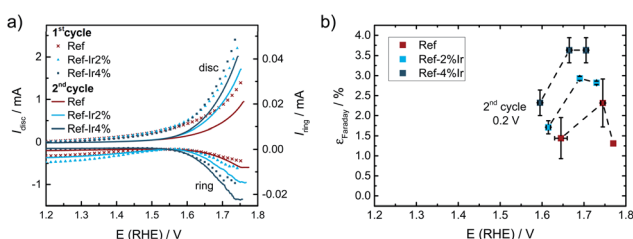
Fig. 10 (a) RRDE measurements to determine the faradaic efficiency for the OER in the overall oxidative current at i_{\text{Disc}} , i_{\text{Ring}} was kept at 0.4 V and 0.2 V during the first and second cycle; respectively, and relates to the ORR. In (b) the faradaic efficiencies for 1 mA cm -2 , 3 mA cm -2 and 5 mA cm -2 are provided for the 2nd scan. All measurements in N 2 saturated 0.1 M H 2 SO 4 at a loading of 0.13 mg cm -2 .
