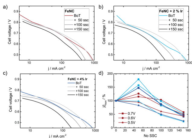
Fig. 12 Fuel cell polarization curves in \text{H}_2/\text{O}_2 at 80 °C for (a) Ref, (b) Ref-2% Ir and (c) Ref-4% Ir at a cathode catalyst loading of 3.5 mg \text{cm}^{-2} (both Ir added catalysts), 4.1 mg \text{cm}^{-2} for Ref. Measurements were made with 1 bar backpressure and a Nafion 212 membrane. In (d) the change in current density at cell voltages of 0.7, 0.6 and 0.5 V is given. The provided curves are averaged values out of two individual measurements. SSCs were performed with \text{H}_2 gas flow at the anode and \text{N}_2 gas flow at the cathode.
