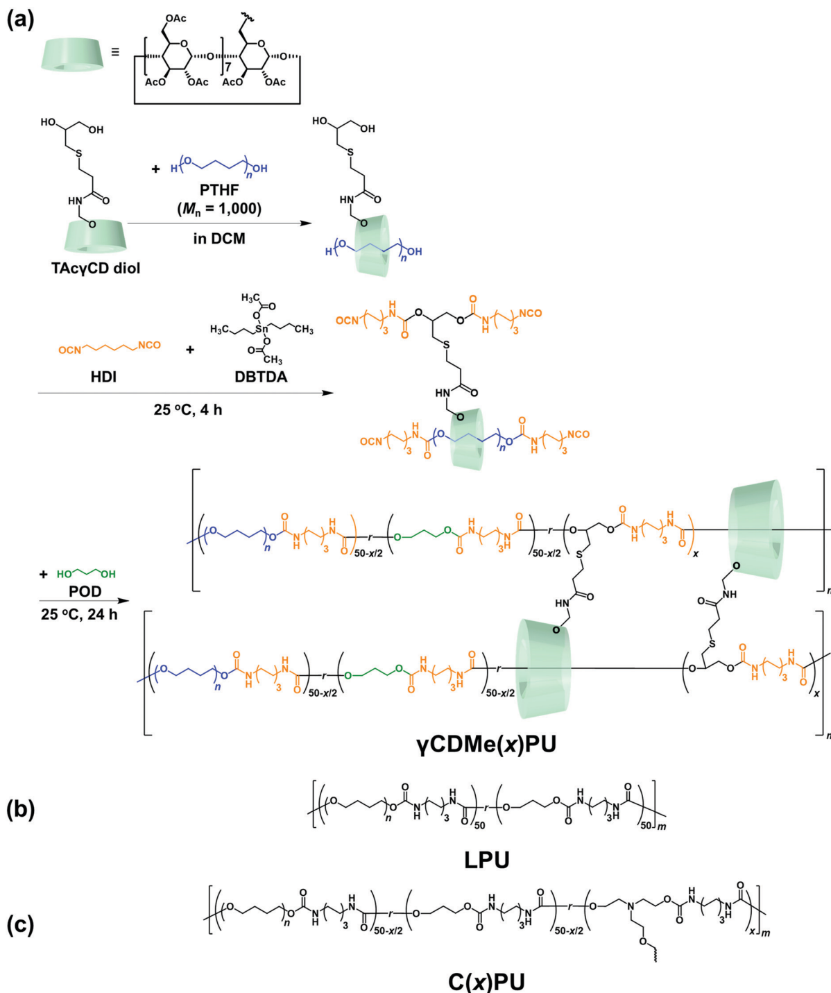
Fig. 1 (a) Synthesis of \gamma\text{CDMe}(x)\text{PU} and chemical structures of (b) LPU and (c) C(x)PU, where x refers to the molar ratio of TAc \gamma\text{CD} diol monomer or TEA monomer.
