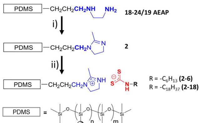
Fig. 2 General pathways for syntheses of PDMS-based ionomers (R = -C_6H_{13} or -C_{18}H_{37} ) from PDMS-based copolymers with randomly distributed N -propylethylenediamine groups (AEAP): (i) 2.0 M dimethylamine and N,N -dimethylacetamide dimethyl acetal (DMADA) in THF under N 2 at room temperature; (ii) hexylamine or octadecylamine and CS 2 in CHCl 3 at 0 °C. The filled black sphere represents an imidazolium group on a PDMS backbone; n = 18–24% of the monomer units within a chain.
