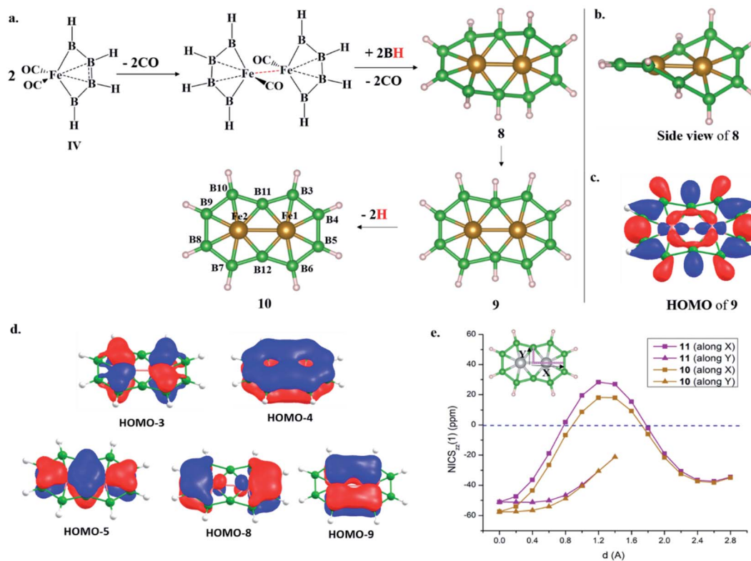
Fig. 2 (a) The design principle of \text{Fe}_2\text{@B}_{10}\text{H}_{10} ( 8 ) and \text{Fe}_2\text{@B}_{10}\text{H}_8 ( 10 ), starting from a B–B homocatenated complex (IV, R = H); planar \text{Fe}_2\text{@B}_{10}\text{H}_{10} ( 9 ) is not a minimum. (b) A side view of \text{Fe}_2\text{@B}_{10}\text{H}_{10} ( 8 ). (c) The HOMO of 9 . (d) The five \pi -MOs of 10 . (e) NICS zz (1) scan curves of 10 and 11 with the distance ( d ) increasing from the top of the ring center towards the periphery along X and Y directions.
