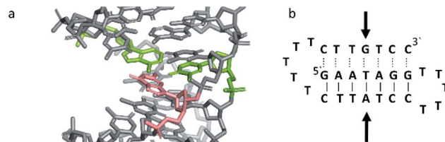
Fig. 7 (a) 3D and (b) schematic representations of the G–T:A triplet of the triplex B. Green indicate the duplex bases, guanine and adenine, while the orange base is the thymine of the TFQ.
