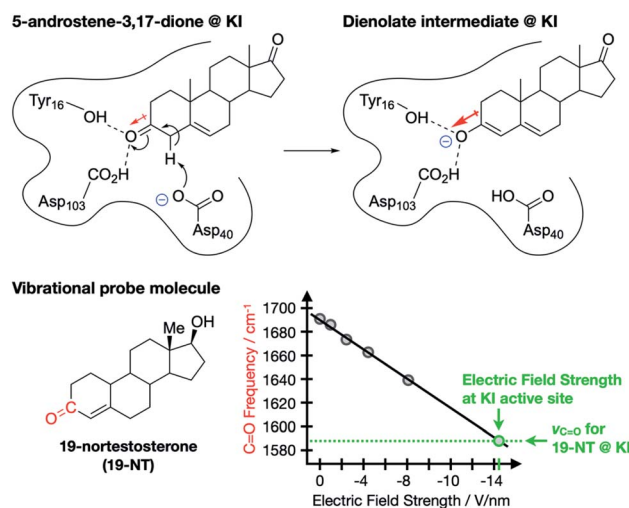
Fig. 2 Enolization reaction of 5-androstene-3,17-dione occurring at the active site of ketosteroid isomerase (KI). 9,11 Red arrows indicate dipole moments associated with the C=O and C–O bonds. 19-nortestosterone was used as a vibrational probe for measuring local ESF strengths via Stark spectroscopy.
