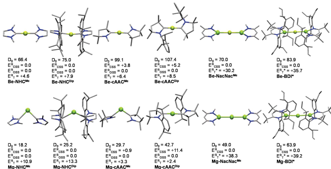
Fig. 1 Optimized ground state geometries (B3LYP-D3(BJ)/def2-SVP), dissociation energies ( D_0 ) (B3LYP-D3(BJ)/def2-TZVP//B3LYP-D3(BJ)/def2-SVP) considering the EL_2 \rightarrow E(0) + 2L(0) dissociation, relative electronic energy for the closed shell singlet ( E_{CSS}^R ), open-shell singlet ( E_{OSS}^R ) and triplet ( E_T^R ) at the B3LYP/def2-TZVP level. *Vertical E_T values. Energies are in kcal mol -1 . Hydrogen atoms were omitted for clarity.
