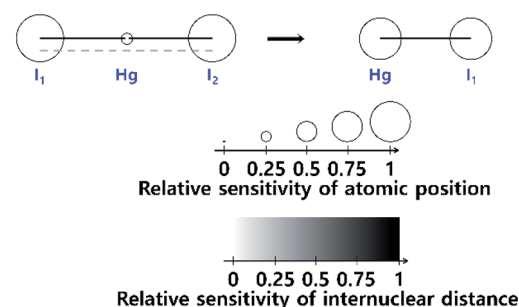
Fig. 1 A sensitivity plot for the dissociation reaction of \text{HgI}_2 , in which \text{HgI}_2 dissociates into \text{HgI} and \text{I} radicals. A sensitivity plot visualizes the relative sensitivities of the atomic positions and internuclear distances to a TRXL signal. The relative sensitivity of the atomic position is indicated by the radius of the sphere, and the relative sensitivity of each internuclear distance is indicated by the color of the line. As the relative sensitivity increases, the radius of a sphere increases, or the color of a line becomes darker. Reproduced from ref. 100 with the permission of John Wiley & Sons, copyright 2022.
