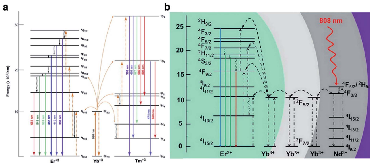
Fig. 1 Proposed energy transfer mechanism showing the UCL processes in (a) \text{Er}^{3+} , \text{Tm}^{3+} , and \text{Yb}^{3+} doped UCNPs under 980 nm laser excitation 31 and (b) \text{Nd}^{3+} , \text{Yb}^{3+} , and \text{Er}^{3+} doped UCNPs under 808 nm laser excitation. 32 Adapted from ref. 31 with permission from Elsevier Ltd, copyright 2014; adapted from ref. 32 with permission from American Chemical Society, copyright 2016.
