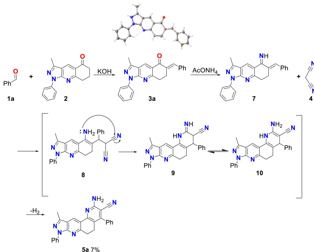
Scheme 2 Mechanism by method A of 2-amino-10-methyl-4,8-diphenyl-6,8-dihydro-5H-pyrazolo[3,4-j][1,7]phenanthroline-3-carbonitrile (5a).
