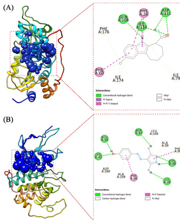
Fig. 3 The active site of each receptor: (A) 415-415I and (B) F18-3TNH.
