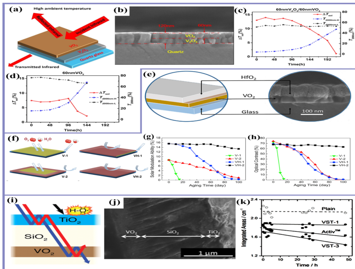
Fig. 6 (a) Experimental flow chart for the synthesis of the \text{V}_2\text{O}_3/\text{VO}_2 bi-layer structure and (b) SEM images of the \text{V}_2\text{O}_3/\text{VO}_2 bi-layer structure. (c) Transmittance spectra of 60 nm \text{VO}_2 at different times in hours. (d) 60 nm \text{VO}_2 at different times in hours. Reproduced with permission 107 Copyright © 2018, Elsevier. (e and f) Flow chart for the whole process of \text{VO}_2/\text{HfO}_2 thin films by using the sputtering method and SEM images. (g) Graph of solar modulation ability versus aging time. (h) Durability of the fabricated films with the graph between optical contrast and aging time (days). Reproduced with permission 108 Copyright © 2019, Elsevier. (i) Preparation of \text{VO}_2/\text{SiO}_2/\text{TiO}_2 thin layers. (j) TEM images of \text{VO}_2/\text{SiO}_2/\text{TiO}_2 thin layers. (k) Durability graph of the \text{VO}_2/\text{SiO}_2/\text{TiO}_2 thin film. Reproduced with permission 109 Copyright © 2016, American Chemical Society.
