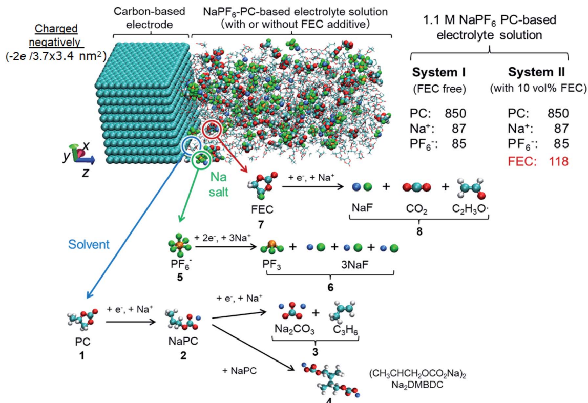
Fig. 1 Model simulation system and reaction schemes in the PC-based electrolyte. (cyan: C, red: O, white: H, orange: P, green: F, blue: Na + ).
