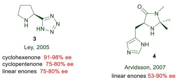
Scheme 4 Conjugate additions using pyrrolidines and imidazolidine catalysts.
