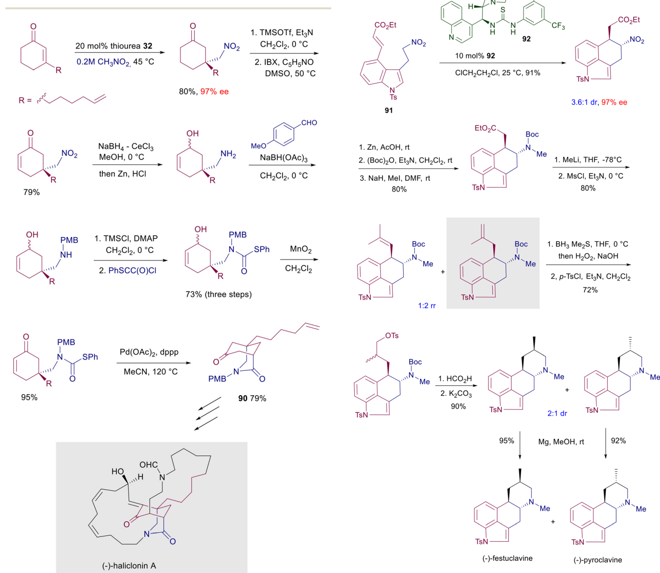
Scheme 69 Synthesis of the ergot alkaloids (–)-festuclavine and (–)-pyroclavine.
