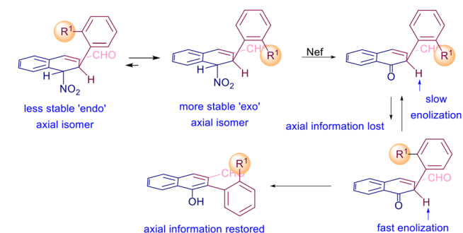
Scheme 15 Enantioselective synthesis of optically active biaryls catalyzed by 11 .
