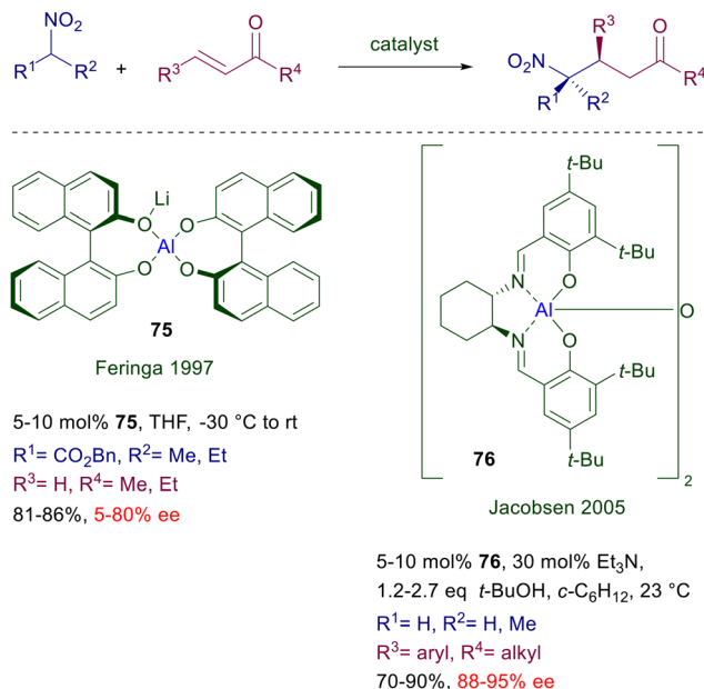
Scheme 56 Asymmetric conjugate additions catalyzed by Al(III) complexes.
