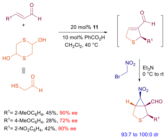
Scheme 12 Synthesis of nitrocyclopropane derivatives.
