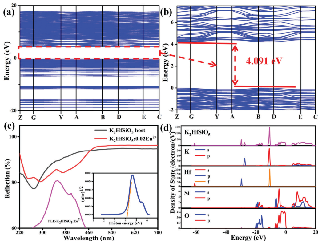
Fig. 3 (a) and (b) Band structure of K 2 HfSiO 5 ; (c) the DRS spectra of Eu 2+ doped and host of K 2 HfSiO 5 (the inset shows the relationship between photon energy and (\alpha h\nu)^{1/2} of the K 2 HfSiO 5 host); (d) total and partial density of states of K 2 HfSiO 5 .
