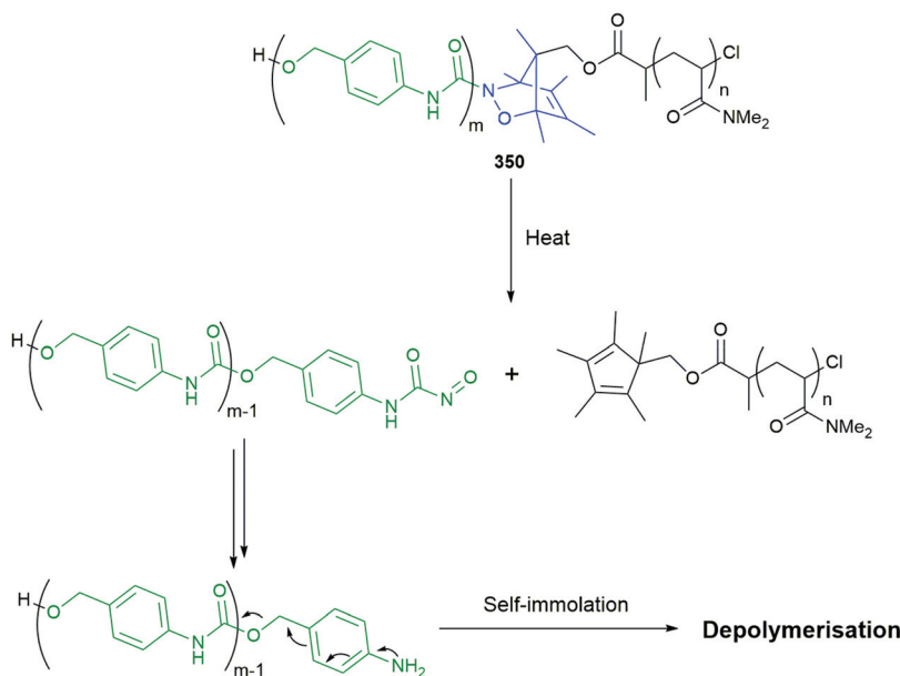
Scheme 84 The self-immolative polybenzylcarbamate-PDMA block copolymer 350 reported 306 by Peterson et al. featuring a temperature sensitive oxazone linker unit which can be degraded thermally to permit self-immolation of the polybenzylcarbamate block.
