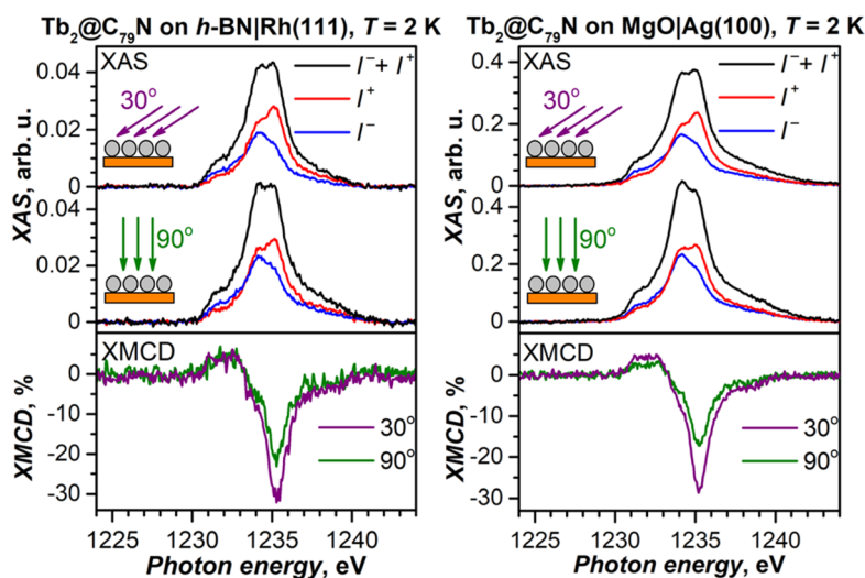
Fig. 8 Tb-M 5 XAS (top panels) and XMCD (bottom panels) spectra of \text{Tb}_2@C_{79}N evaporated onto h-BN|Rh(111) (left) and MgO|Ag(100) (right). T \approx 2 K, \mu_0H = 6.8 T, grazing (30°) and normal (90°) X-ray and magnetic field incidence with respect to the surface. I^+ and I^- are circular polarized XAS spectra, non-polarized XAS is defined as a sum ( I^+ + I^- ), XMCD is defined as a difference ( I^- - I^+ ), normalization to the maximum of XAS gives XMCD in %.
