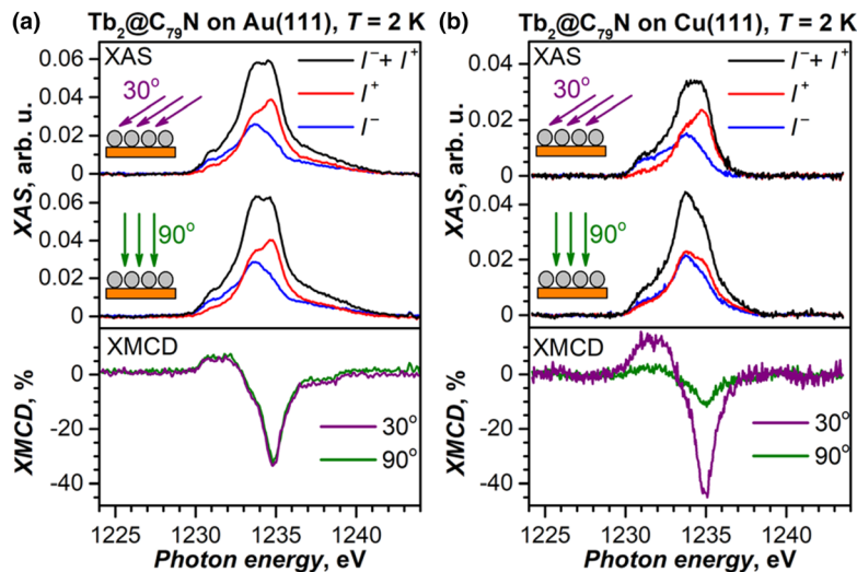
Fig. 6 Tb- M_5 XAS (top panels) and XMCD (bottom panels) spectra of Tb 2 @C 79 N submonolayers (~0.2 ML coverage) on Au(111) (a) and Cu(111) (b). T \approx 2 K, \mu_0 H = 6.8 T, grazing (30°) and normal (90°) X-ray and magnetic field incidence with respect to the surface. I^+ and I^- are circular polarized XAS spectra, non-polarized XAS is defined as a sum ( I^+ + I^- ), XMCD is defined as a difference ( I^- - I^+ ), normalization to the maximum of XAS gives XMCD in %.
